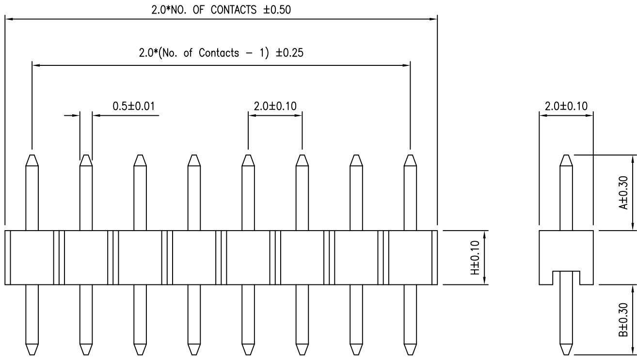
Pin Chart
